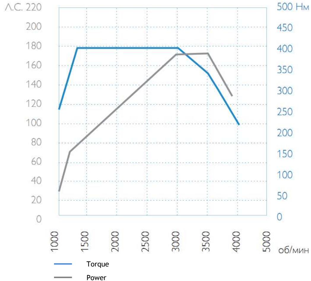
3.0 COMMON RAIL 170 Л.С.
